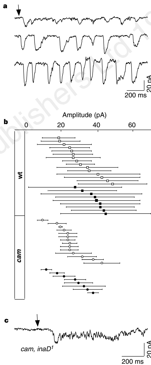
Figure 2 A quantum bump is an organized unit of signalling. a , Single-photon responses from a cam mutant photoreceptor. Each trace represents quantum bumps produced by a single activated photoreceptor; the three different traces represent the activity produced by three different rhodopsin molecules. Bath solution contained 0.4 mM CaCl 2 . b , The spread of quantum bumps produced by different activated receptors compared with the spread of bumps produced by one activated receptor. Responses of 24 wild-type (wt) cells and 22 cam mutants are shown. Each trace represents the mean \pm s.d. of seven bumps generated by consecutive flashes of light (wt), or the mean \pm s.d. of seven bumps generated by a single photon of light ( cam ). Cells were stimulated with a 10-ms flash of 580-nm light, \log[I] = -6.5 . The spread of all of the different cam responses mimics the variability seen in normal single-photon responses. The open symbols indicate that the bath solution contained 1.5 mM CaCl 2 , and the filled symbols indicate that the bath solution contained 0.4 mM CaCl 2 . c , Quantum bumps from cam, inaD 1 double mutants show that loss of InaD disrupts localized signalling.
