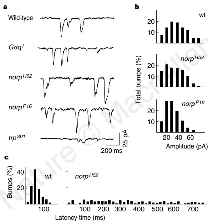
Figure 3 Amplification occurs downstream of PLC activation. a , Quantum bumps from a wild-type photoreceptor, from a photoreceptor containing ~1% of the normal levels of the eye-specific G \alpha subunit ( Gαq 1 ), and from photoreceptors that express reduced levels of PLC ( norpA H52 and norpA P16 ) are shown. Quantum bumps from a photoreceptor with low levels of the light-activated ion channel TRP ( trp 301 ) are also shown; this photoreceptor exhibits significant reduction in bump size 12 . These results indicate that signal amplification occurs at the terminal signalling events, downstream of PLC activation. Stimulation was with continuous light of \log[I] = -7 for wild-type, norpA H52 and trp 301 , and \log[I] = -4 for Gαq 1 . b , Amplitude distributions of quantum bumps in the norpA hypomorphs. For studies with wild-type and norpA H52 alleles, cells were stimulated with a 10-ms flash of 580-nm light of \log[I] = -6.5 . The probability of a bump occurring ( P ) was 0.30 for wild-type and 0.28 for norpA H52 photoreceptors. c , Distributions of latency times for the norpA H52 hypomorph. Latency was measured as the time from the onset of the light stimulus (10 ms, \log[I] = -6.5 ) to the peak amplitude of the response. For the norpA P16 allele, the mean latency time was estimated as ~60 s, derived from the exponential decay of the bump rate following stimulation with a 10-ms flash of light of \log[I] = -4.5 . See Table 1 for quantification of response parameters.
